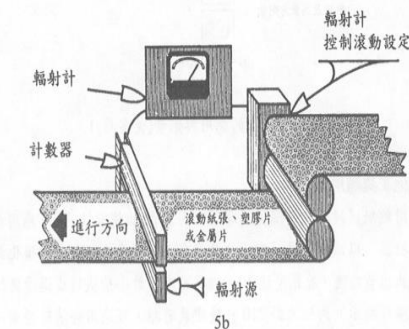
厚度计 Thickness meter
